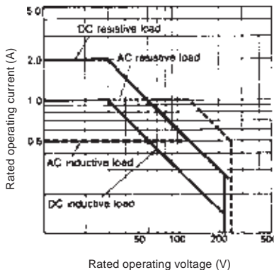
Maximum switching capacity DPDT
